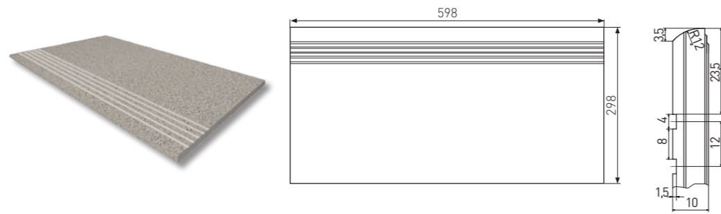
schodovka | step tile | TCPSE... | 298×598×10 mm |
