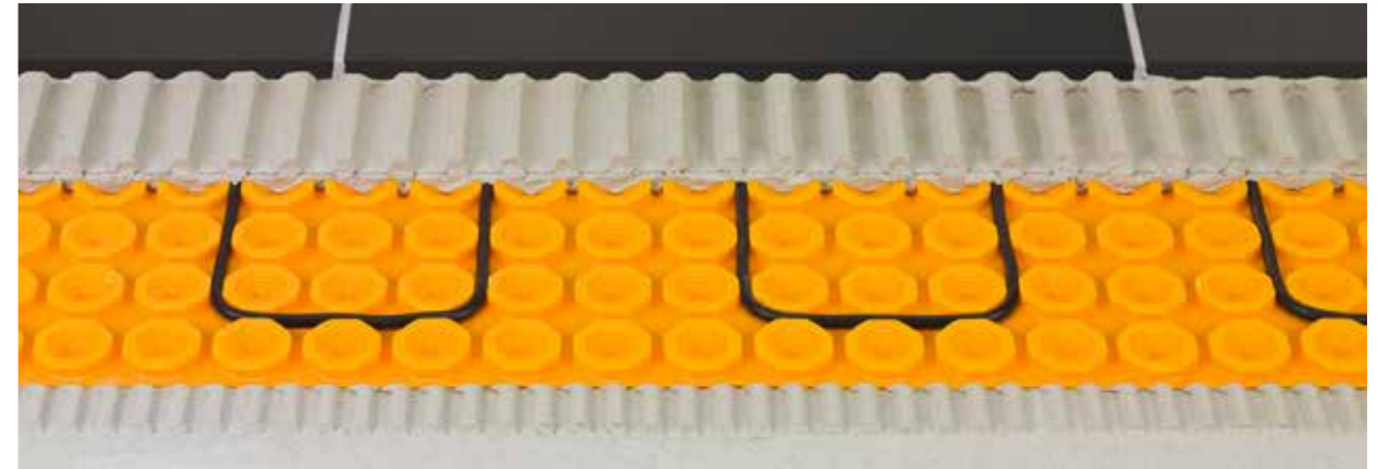
Fig. 14 System of floor heating cables placed on a base plate with a built-up thermal barrier (Fig.: Schlüter-Systems)
