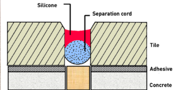
Fig. 27 Flexible expansion joint strip
