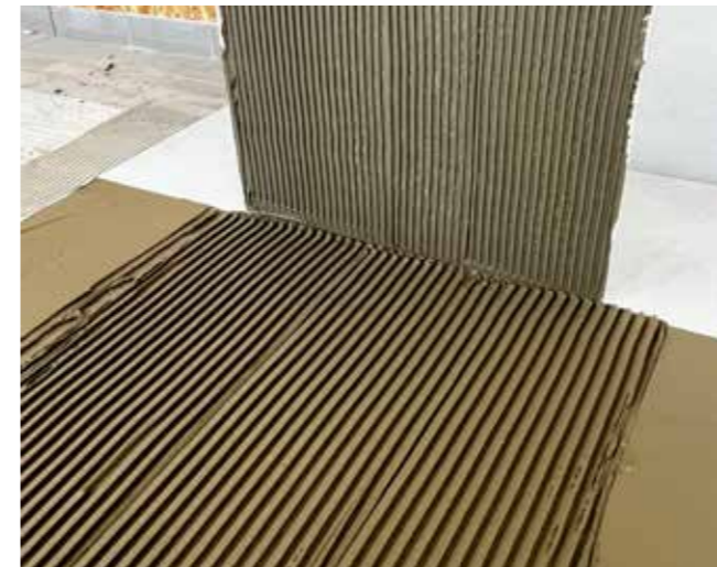
Fig. 10 Buttering-floating bonding
